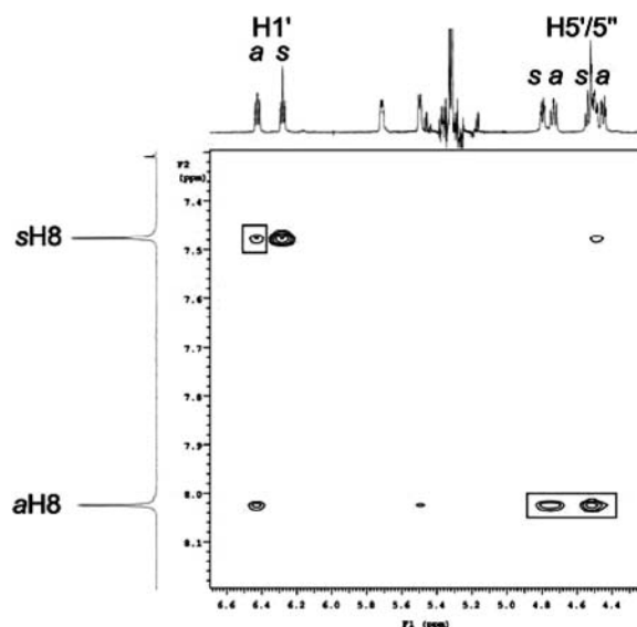
Figure 4. Portion of the 600 MHz NOESY spectrum of the octameric complex between 2b and K-Pic, recorded at rt in \text{CD}_2\text{Cl}_2 (mixing time 150 ms) showing the interquartet correlations.
