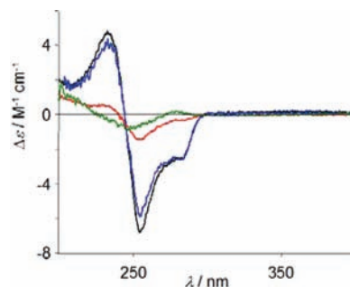
Figure 2. CD spectra of 2a (5 mM) before (red line) and after (black line) K-Pic extraction. CD spectra of 2a /K-Pic complex sample after dilution to 0.5 mM (blue line) and after addition of 4 equiv [2.2.2] cryptand (green line).
