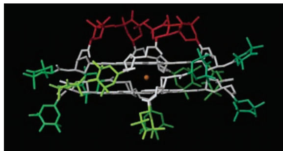
Figure 5. Structure of the octamer that refer to the time interval of dynamic simulation between 2000th to the 2250th ps.
