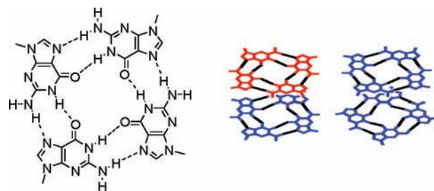
Figure 1. G-quartet motif and a schematic representation of D_4 and C_4 -symmetric octamers. Red and blue color refers to the two heterotopic faces of the G-quartet.
