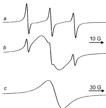
Figure 3. ESR spectra of 2a (0.5 mM) before (a) and after (b) K-Pic extraction. (c) ESR spectrum recorded at 77 K in \text{CH}_2\text{Cl}_2 glass in the presence of \text{K}^+ .
